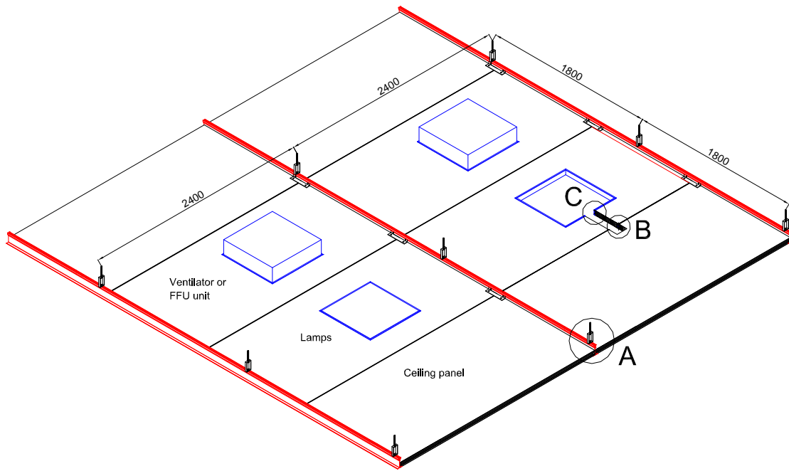
T-grid ceiling model with the main elements
